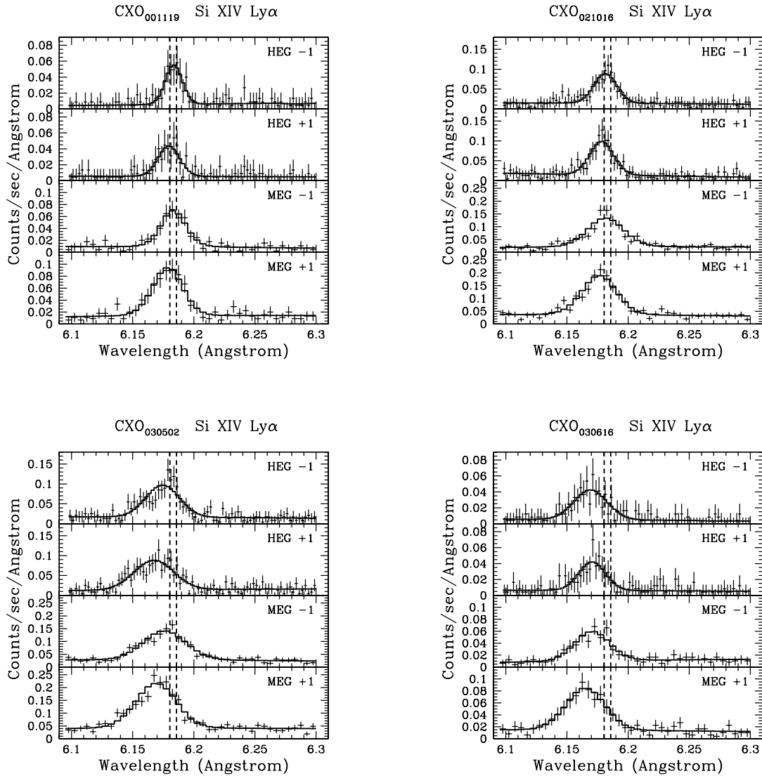
FIG. 8.—As Fig. 7, but showing the Si xiv Ly \alpha line. The vertical dashed lines show the rest wavelengths of the two components of the line (6.1804 and 6.1858 Å, respectively).
