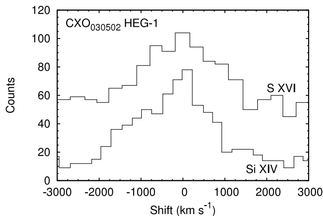
FIG. 13.—Comparison of the HEG -1 profiles of S XVI and Si XIV Ly \alpha from CXO 030502 . For clarity, the profiles have been binned by a factor of 2, and the S XVI profile has been shifted upward by 30 counts.
