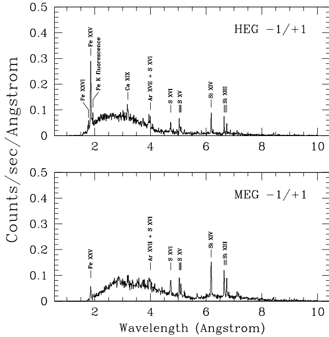
FIG. 1.— Chandra HETGS spectra of \eta Car from CXO 001119 , \phi = 0.528 . For each grating (HEG and MEG) the +1 and -1 orders have been co-added, and the spectra have been binned up to 0.01 Å.
