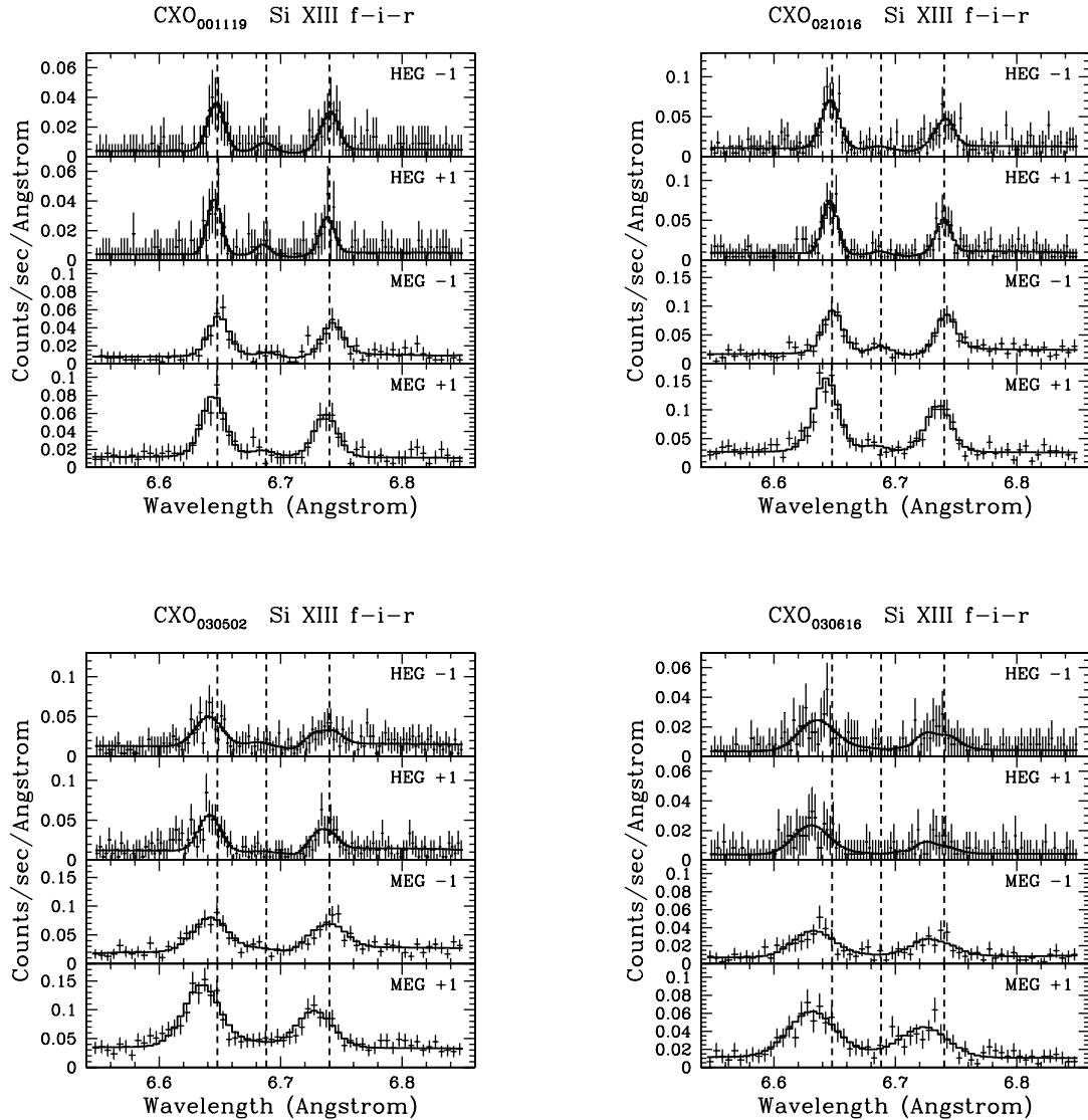
FIG. 7.— Si XIII f-i-r triplets from CXO 001119 , CXO 021016 , CXO 030502 , and CXO 030616 , showing the best-fitting Gaussian line model obtained by fitting to each spectral order individually. The vertical dashed lines show the rest wavelengths of the resonance, intercombination, and forbidden lines (6.6479, 6.6882, and 6.7403 Å, respectively).
