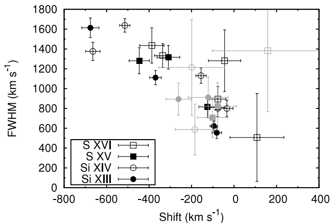
FIG. 10.—Observed emission line widths plotted against the line shifts, showing the correlation between the two. The gray data points are for lines contaminated by the CCE component (Hamaguchi et al. 2007).
