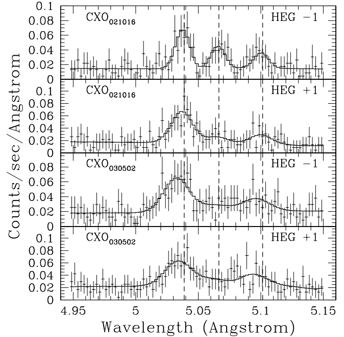
FIG. 14.—First-order HEG spectra of the S xv fi-r triplet from CXO 021016 (top two panels) and CXO 030502 (bottom two panels). The histograms show the best-fitting Gaussian line models obtained by fitting to each spectral order individually. The vertical dashed lines show the rest wavelengths of the resonance, intercombination, and forbidden lines (5.0387, 5.0665, and 5.1015 Å, respectively).
