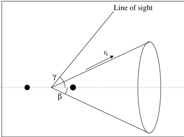
FIG. 16.—Geometrical model of the wind-wind collision in \eta Car. The filled circles represent the two stars. The cone (with opening half-angle \beta ) represents the wind-wind interaction region (along which X-ray-emitting material is streaming at speed v_0 ). The viewing angle \gamma is the angle between the line of sight and the line of centers.
