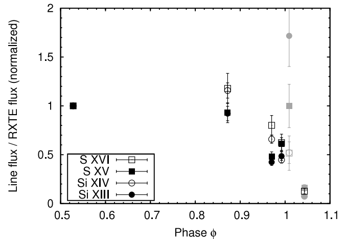
FIG. 12.—Observed emission line fluxes divided by the contemporaneous 2–10 keV flux measured with RXTE (Corcoran 2005). For S XV and Si XIII we use the resonance line flux. For all lines, the flux ratios have been normalized to the values for phase \phi = 0.528 (CXO 001119 ). The gray data points are for lines contaminated by the CCE component (Hamaguchi et al. 2007).
