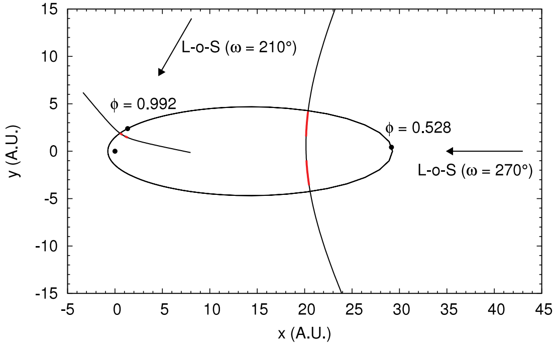
FIG. 22.— Orbit of \eta Car with the eccentricity ( e = 0.95 ) from our line profile modeling. All other orbital parameters are the same as those used in Fig. 17. The arrows show the lines of sight (L-o-S) projected into the orbital plane for two different values of the longitude of periastron; that obtained without including absorption in the model ( \omega = 210^\circ ; see § 5.2) and that obtained when the effects of absorption are included in the model ( \omega = 270^\circ ; see § 5.3). Also shown is a comparison of the stellar orientations and geometry of the contact discontinuity for two phases corresponding to observations CXO 001119 ( \phi = 0.528 ) and CXO 030616 ( \phi = 0.992 ). In each case the red interval shows the approximate x range where the line luminosity l(x) (see eq. [8]) is greater than half its maximum value for the Si xiv line. We plot results for the version of the model which includes the effects of absorption (§ 5.3; lower part of Table 7). The extent of the S xvi emission region is similar to that of the Si xiv emission region.
