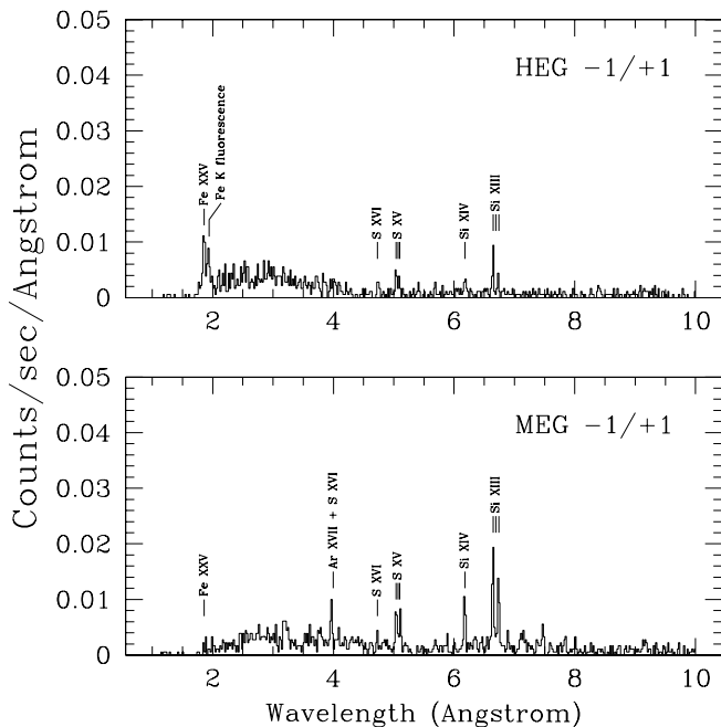
FIG. 5.—As Fig. 1, but for CXO 030720 , \phi = 1.009 , with the spectrum binned up to the 0.02 Å, instead of 0.01 Å. Note that the y-axis range is different from Figs. 1–4 and 6.
