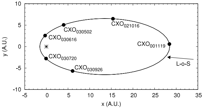
Fig. 17.—Orbit of \eta Car's companion plotted in the rest frame of the primary (marked with an asterisk at the origin). The positions of the companion at the times of the Chandra HETGS observations are marked with black circles. The arrow shows the line of sight (L-of-S) projected into the orbital plane. This orbit was plotted using the parameters in Table 6. The length scale of the orbit is set by assuming masses of 80 and 30 M_{\odot} for the primary and the companion, respectively (Corcoran et al. 2001a).
