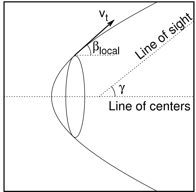
FIG. 20.—Diagram showing the geometry used in the line profile calculations. Each point along the wind-wind collision surface represents a ring of expanding material, comprising material flowing tangentially along the wind-wind collision surface at speed v_t . Locally, the flow velocity makes an angle \beta_{\text{local}} with the line of centers, while the line of sight makes an angle \gamma with the line of centers. Note that the curvature of the surface has been exaggerated for clarity.
