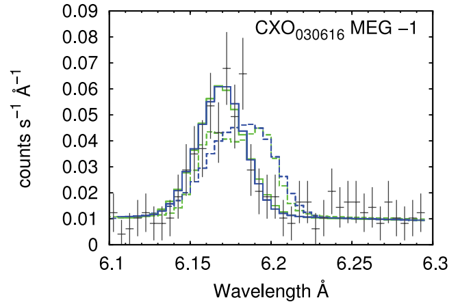
FIG. 23.—Model Si XIV profiles with (solid curves) and without (dashed curves) absorption, compared with the MEG -1 Si XIV line from CXO 030616 . As in Fig. 21, the green profiles were calculated with \omega = 270^\circ , i = 50^\circ , and the blue profiles with \omega = 180^\circ , i = 50^\circ .
