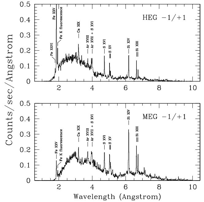
FIG. 2.— As Fig. 1, but for CXO 021016 , \phi = 0.872 .
