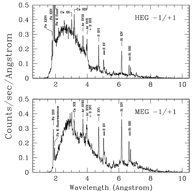
FIG. 3.— As Fig. 1, but for CXO 030502 , \phi = 0.970 .
