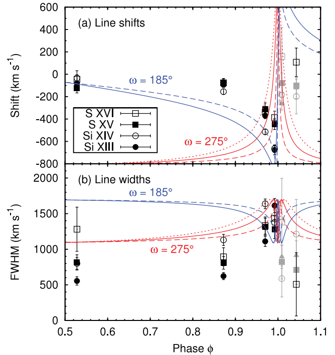
Fig. 18.—Comparison of the predictions of the simple geometrical model (§ 4) with the observed line shifts and widths. The solid red curves were generated from the orbital parameters in Table 6 ( i = 50^{\circ} , \omega = 275^{\circ} , e = 0.9 ). The other red curves show the effect of varying the eccentricity: e = 0.85 (short dashed curve) and e = 0.95 (long dashed curve). The blue curves show the effect of adjusting \omega to 185^{\circ} , for two different eccentricities: e = 0.9 (solid curve) and e = 0.95 (long dashed curve). The gray data points are for lines contaminated by the CCE component (Hamaguchi et al. 2007).
