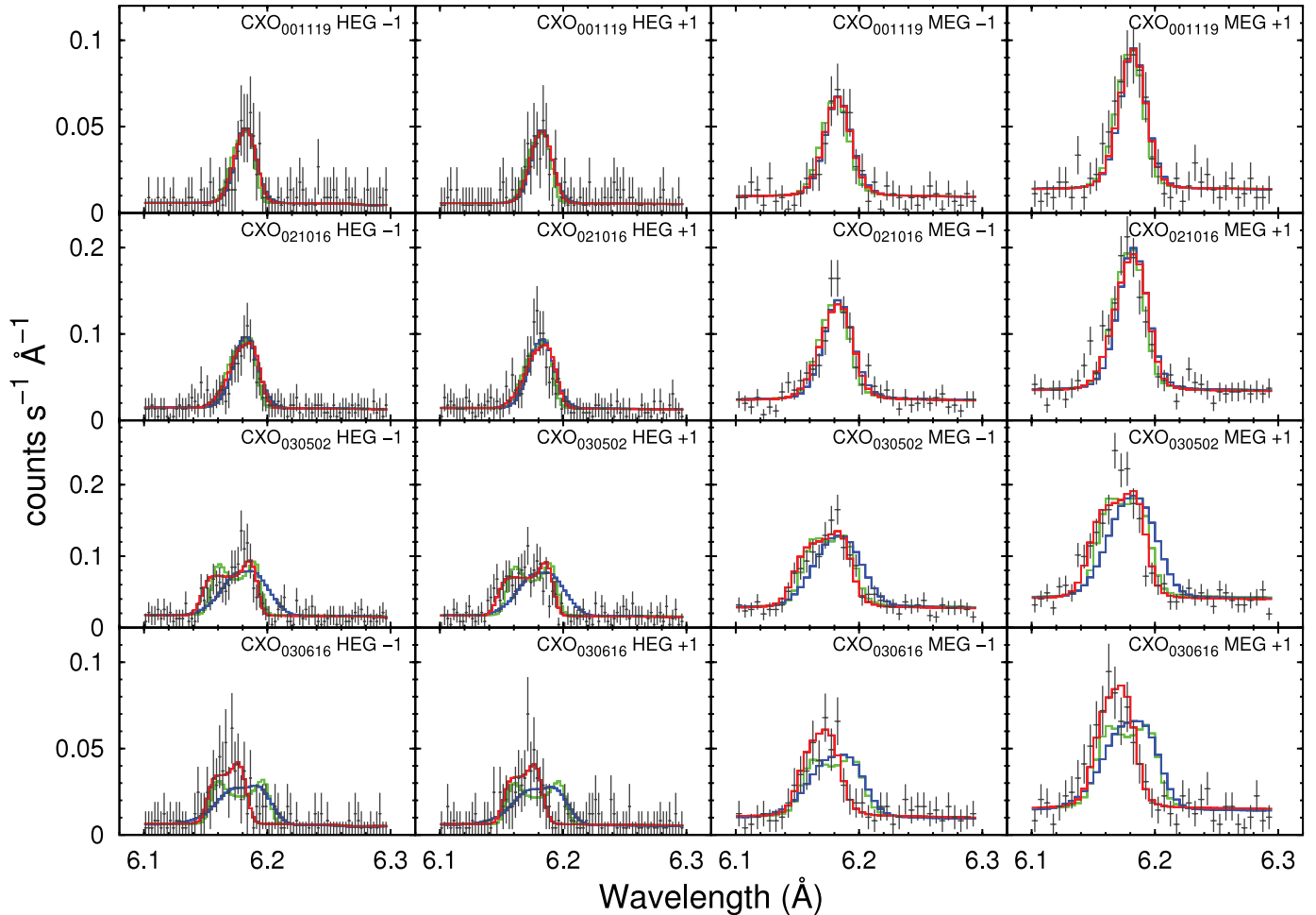
FIG. 21.— Comparison of our model profiles with the observed Si XIV Ly \alpha lines, from CXO 001119 , CXO 021016 , CXO 030502 , and CXO 030616 (plotted from top to bottom). Each spectral order is plotted separately. The red curves show the profiles calculated with \omega = 210^\circ , i = 70^\circ ; the green curves the profiles calculated with \omega = 270^\circ , i = 50^\circ ; and the blue curves the profiles calculated with \omega = 180^\circ , i = 50^\circ .
