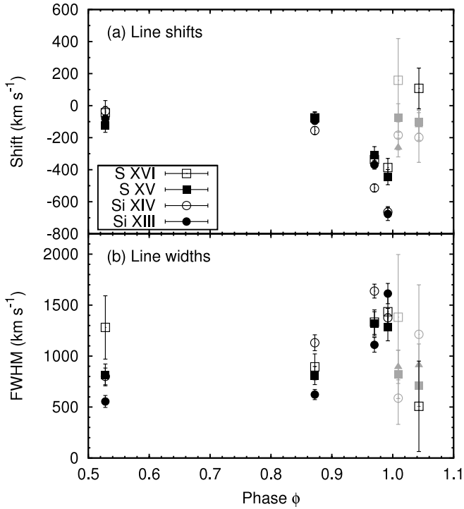
FIG. 9.—Observed emission line (a) shifts and (b) widths plotted against phase. The phase for each observation is taken from Table 1. Phase \phi = 1 corresponds to the start of the X-ray minimum in 2003 June. The gray data points are for lines contaminated by the CCE component (Hamaguchi et al. 2007).
