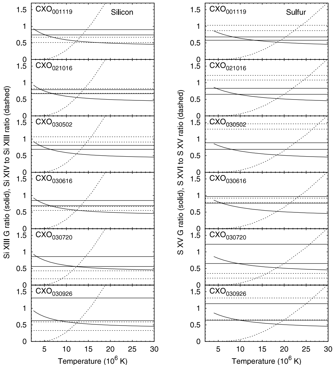
FIG. 15.— G = [(f + i)/r] line flux ratios and H-like to He-like line flux ratios for silicon ( left ) and sulfur ( right ). The horizontal solid lines show the observed values of G ( 1 \sigma limits), while the curved solid lines show the theoretical values as a function of temperature from APED. The dashed lines show similar information for the flux ratio of the H-like Ly \alpha line to the He-like resonance line. (For the latter ratio we use the flux of the brighter component of the Ly \alpha doublet.)
