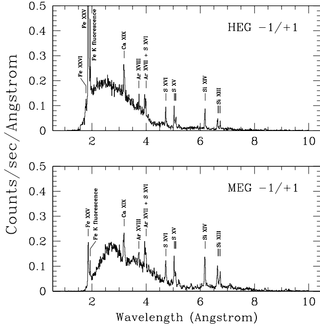
FIG. 4.—As Fig. 1, but for CXO 030616 , \phi = 0.992 .
