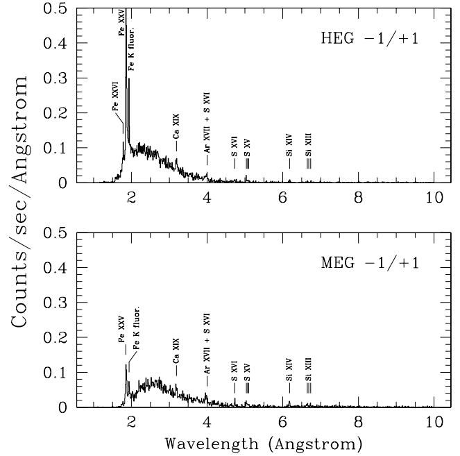
FIG. 6.—As Fig. 1, but for CXO 030926 , \phi = 1.043 .
