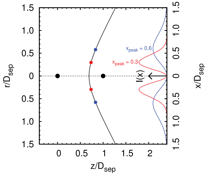
FIG. 19.—Shape of the wind-wind collision surface in \eta Car, calculated using the equations of Cantó et al. (1996). The two stars are shown by the black circles on the z -axis: the primary is at the origin, and the companion is at (1, 0) . Distances are normalized to the stellar separation D_{\text{sep}} . The curves to the right show l(x) (see eq. [8]) plotted for two different values of x_{\text{peak}} : red curves: x_{\text{peak}} = 0.3 ; blue curves: x_{\text{peak}} = 0.6 . Note that x is actually the distance measured along the wind-wind collision surface. The points at x = 0.3 and x = 0.6 are marked on the surface with the red and blue circles.
