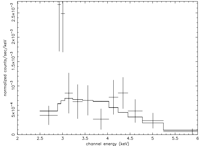
Fig. 1. A plot of counts per second per keV versus energy for the data (crosses) and best-fitting model (solid line).
