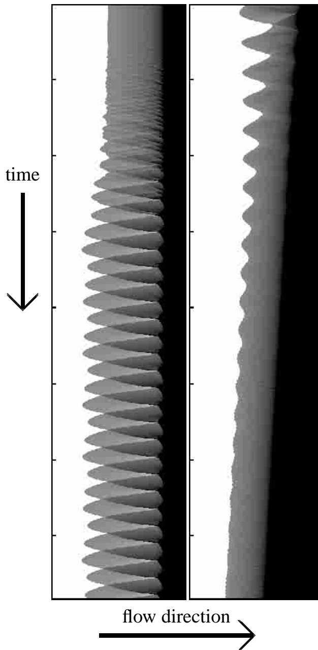
Fig. 1. Spacetime diagrams of a radiative shock for M = 10 , \alpha = 0.0 (cf. Fig. 3 in Strickland & Blondin 1995). The tick marks on the vertical axis are in units of 25L_c/v_0 where L_c is the cooling length of the shock (see Strickland & Blondin 1995). The width of the horizontal axis is 1.88L_c . The supersonic flow enters the grid from the left, and the cooled postshock gas flows off the grid to the right. The grayscale shows the density of the gas, with lighter shades signifying diffuse gas and darker regions denoting higher density. In the left panel, q_0 = 0 , and the system exhibits linear growth for the first \sim 40\% of the run. In the right panel, where q_0 = 150 , the initial conditions are far from equilibrium for a mass-loaded shock, and the system exhibits powerful oscillations, though these are quickly damped as expected from the linear stability analysis in Sect. 2.
