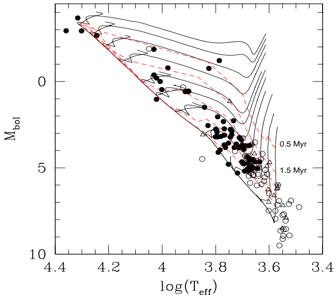
Fig. 8. Hertzsprung-Russell diagram of the X-ray selected stars in NGC 6530. Evolutionary tracks from Siess et al. (2000) for masses of 0.5, 0.7, 1.0, 1.5, 2.0, 2.5, 3.0, 4.0, 5.0, 6.0 and 7.0 M_{\odot} are overplotted. Filled symbols indicate X-ray detected objects without H\alpha emission, whereas encircled asterisks stand for PMS stars selected from their H\alpha emission. The open circles and open triangles stand for H\alpha selected PMS and PMSc stars from Sung et al. (2000) respectively. The thick solid line shows the ZAMS, while the dashed lines correspond to isochrones for ages of 0.5, 1.5, 4.0, 10.0 and 20.0 Myr (for clarity only the first two isochrones are labelled).
