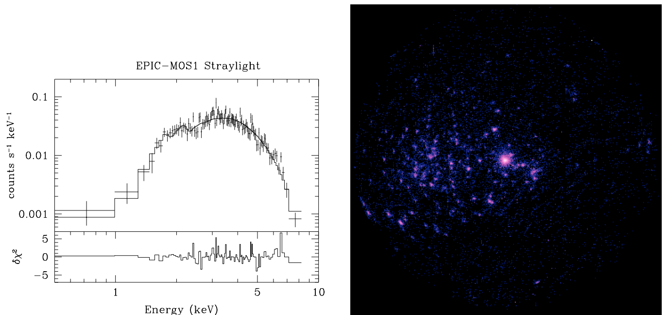
Fig. 2. Left panel: spectrum of the brightest straylight feature in the EPIC-MOS1 image. The energy distribution can be fitted with a heavily absorbed ( N_{\text{H}} = (3.1 \pm 0.3) \times 10^{22} \text{ cm}^{-2} ) blackbody model of temperature kT = 1.04 \pm 0.05 \text{ keV} . Right panel: combined EPIC MOS1 + MOS2 image extracted over the PI range from 200 to 1500. The image is displayed with a logarithmic scale. The faint sources near 9 Sgr are associated with the young open cluster NGC 6530 inside the Lagoon Nebula. These sources are discussed in a separate paper.
