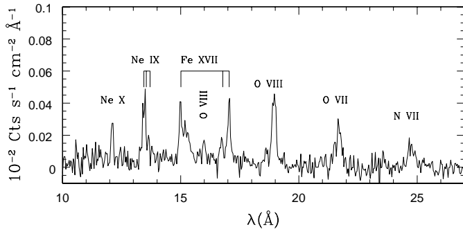
Fig. 3. Combined RGS1+2 first order spectrum of 9 Sgr.
