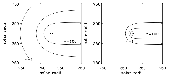
Fig. 3. Contours of optical depth at 6 cm in the stellar wind of an O5 V star (left panel) and an O8 V star (right panel). The observer is situated to the left. The contour lines of \tau = 1, 10 and 100 are shown. The two dots indicate the position of both components of the binary.
